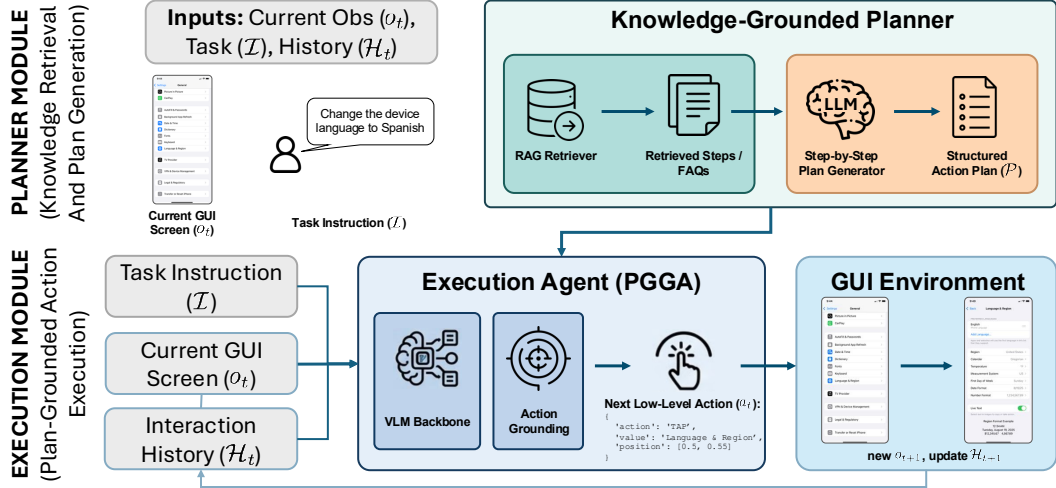
Figure 1: Plan-Grounded GUI Agent (PGGA) Framework. Given a natural language task and the current visual state, an intermediate Planner module queries an external Knowledge Base to retrieve relevant documentation and synthesizes it into a step-by-step Action Plan. The model then predicts the next action by heavily conditioning on this explicit procedural plan, alongside the original task, current screenshot, and interaction history.
