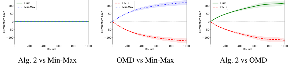
Figure 2: All vs all comparison for T = 1000 rounds. The x-axis displays the round t , and the y-axis displays how much the respective algorithm (Min-Max, OMD, Algorithm 2) gained from the other.
