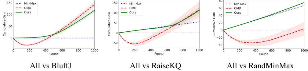
Figure 3: All vs Bob comparison for T = 1000 rounds. The x-axis displays the round t , and the y-axis displays how much Min-Max, OMD, and Algorithm 2 gained from the second algorithm so far. The y-axes have varying scales for readability.
