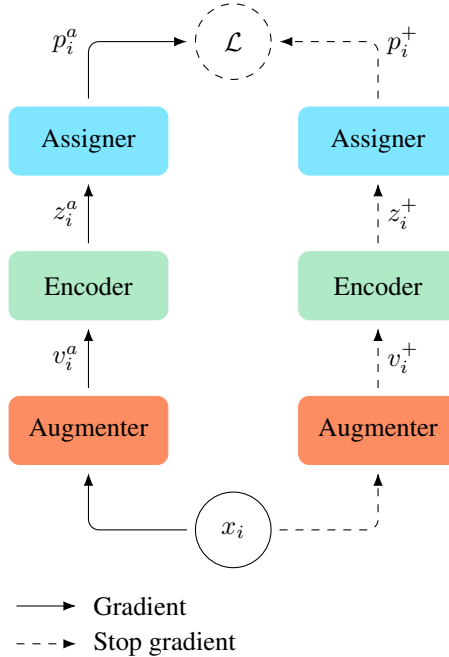
Figure 1: An observation x_i gets transformed into two stochastic views, v_i^{(\cdot)} , that are further encoded into a representation space, z_i^{(\cdot)} . We obtain a distribution, p_i^{(\cdot)} , of the representations’ assignments to a set of clusters. Our objective \mathcal{L} is to compare these distributions and minimize their difference. We use one view as an anchor (superscripted by a ) that is trained, while another positive view (superscripted by + ) that is not.
