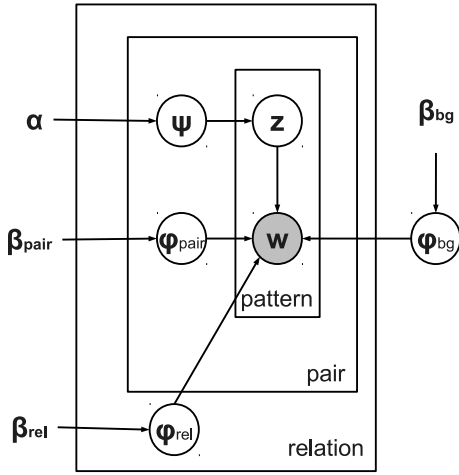
Figure 2: Hierarchical topic model for distant supervision. Context patterns are generated by either a background, relation-specific or pair-specific distribution.
