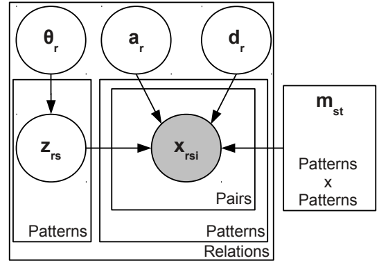
Figure 3: Plate diagram representing the Takamatsu model, according to [17]. The hidden variables z_{rs} indicate whether a relation r is expressed by a pattern s . The observed variables x_{rsi} denote which contexts are matched by an argument pair i . \theta_r, a_r and d_r are the parameters to be learned, m contains the correlation statistics.
