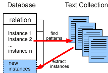
Figure 1: Distant supervision for knowledge base population.
