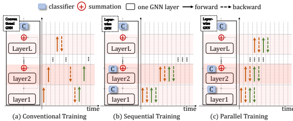
Figure 2: Signal propagation process for conventionally trained GNN, sequentially trained layerwise GNN, and the parallel trained GNN. Arrows of different colors represents different batches of data (can be either mini-batch or full-batch). We assume the forward process and backward process have the same time cost, we also assume the auxiliary classifier computation is negligible, these are only for simpler illustration purposes.
