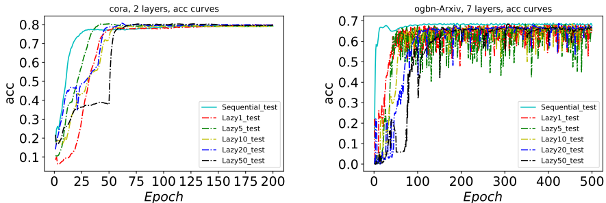
Figure 3: Comparison of sequential and parallel training. Results show that parallel can quickly catches up to sequential training within a few epochs.
