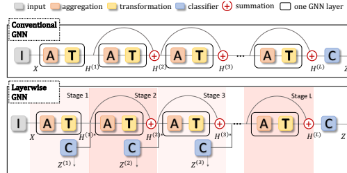
Figure 1: High level framework of conventional deepGCN (upper) and layerwise deepGCN (lower). The aggregation step (A) corresponds to FH^{(l-1)} operation and the transformation step corresponds to \sigma(\cdot W^{(l)}) operation. In conventional training, both steps are done for every iteration, but for sequential layerwise training, we can decouple these two operations to conduct the transformation step in every iteration, but the aggregation step only once at the beginning of each layer, which results in the demonstrated time saving.
