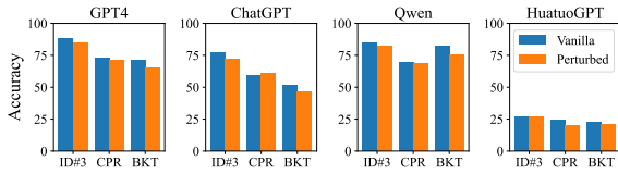
Figure 6: Robustness test of GPT4, ChatGPT, Qwen, and HuatuoGPT on different datasets.
