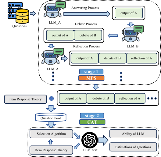
Figure 9: The workflow of Agent-based CAT
