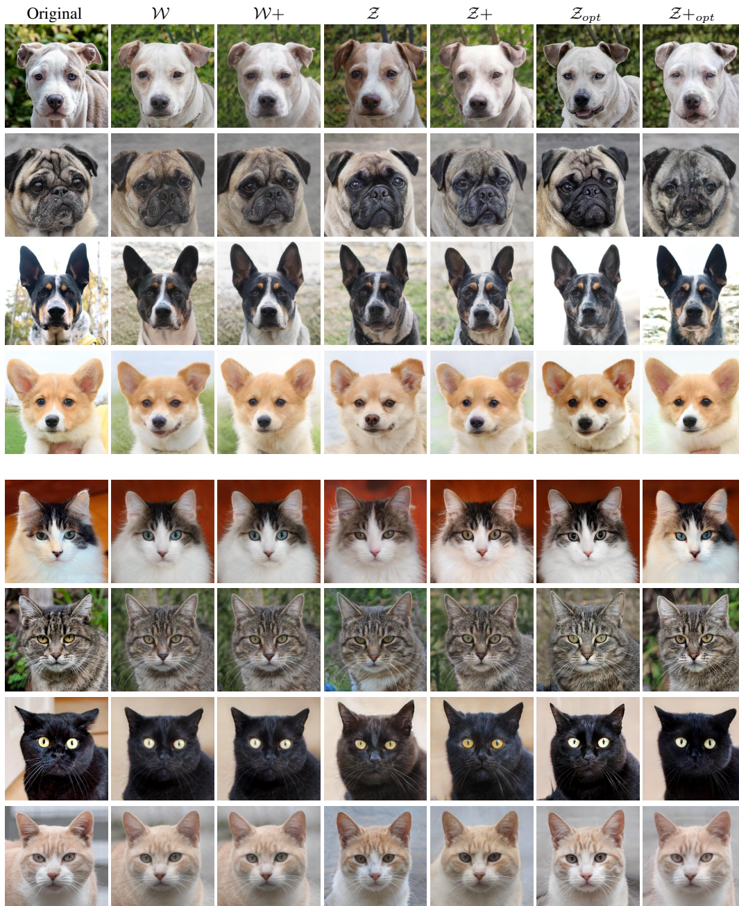
Figure 16: To invert real images of animal faces to different latent spaces, we examine both encoders and latent optimization based methods. We use the pSp encoder (Richardson et al., 2021) as a backbone and modify it to embed into \mathcal{W} , \mathcal{Z} , and \mathcal{Z}+ (Song et al., 2021) spaces. For the \mathcal{W}+ space, we use e4e (Tov et al., 2021), which also uses pSp (Richardson et al., 2021) as backbone. For optimization based inversion, we modify the optimization code from StyleGAN2 (Karras et al., 2020b) to \mathcal{Z} or \mathcal{Z}+ space (two rightmost columns). All of the inversion methods yield reasonably faithful reconstructions, with occasional artifacts in the \mathcal{Z} and \mathcal{Z}_{opt}+ reconstructions. Note that, as we show below, that better reconstruction does not necessarily yield the best image translation.
