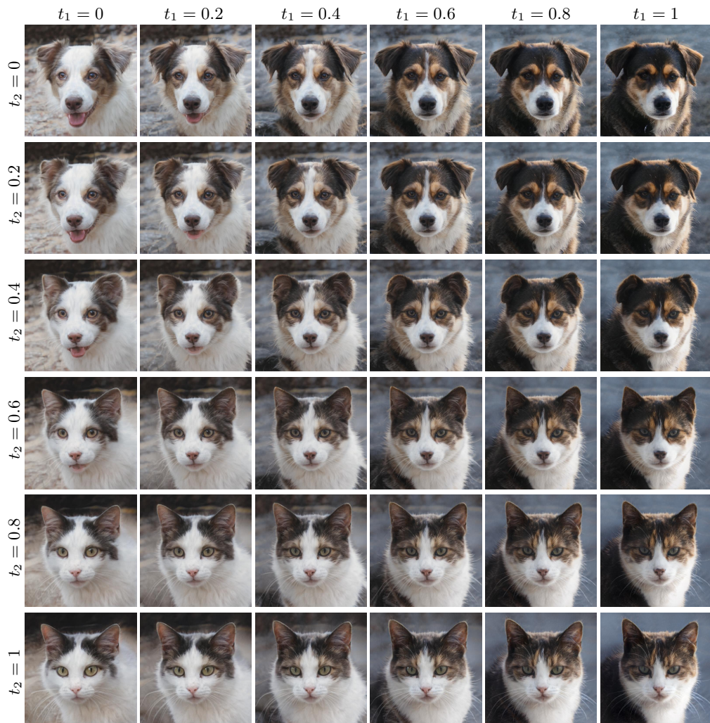
Figure 25: Given a pair of real images from domain A (top-left) and B (bottom-right), we smoothly transition between them by interpolating their latent codes in \mathcal{W}_+ , as well as the model weights. t_1 is the interpolation coefficient for the latent codes, while t_2 is the coefficient for the model weights. In the same column (fixed t_1 ), we obtain a smooth transition between the domains (different species, but the same pose and fur color). In the same row (fixed t_2 ), we have a smooth transition inside the same domain (same species, varying pose and fur color). Any trajectory between the top-left and bottom-right corners yields a smooth morph sequence between two input images. See the accompanying video, which progresses along the diagonal t_1 = t_2 .
