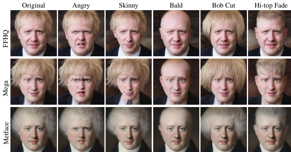
Figure 10: Semantic alignment of multiple channels: semantically meaningful directions in StyleSpace discovered in the parent model (FFHQ), detected using StyleCLIP (Patashnik et al., 2021), still control the same attributes in children models (Mega and Metface).
