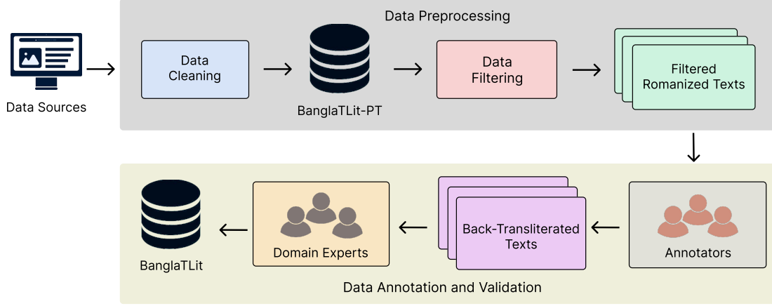
Figure 2: Pipeline of creating BanglaTLit-PT and BanglaTLit datasets. The data collected from various sources are aggregated and thoroughly cleaned to produce the BanglaTLit-PT corpus. The corpus is filtered, annotated, and verified by domain experts to create the BanglaTLit transliteration dataset.
