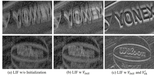
Figure 7. Visualization of the neuron responses of different configurations under MS-RBD dataset.
