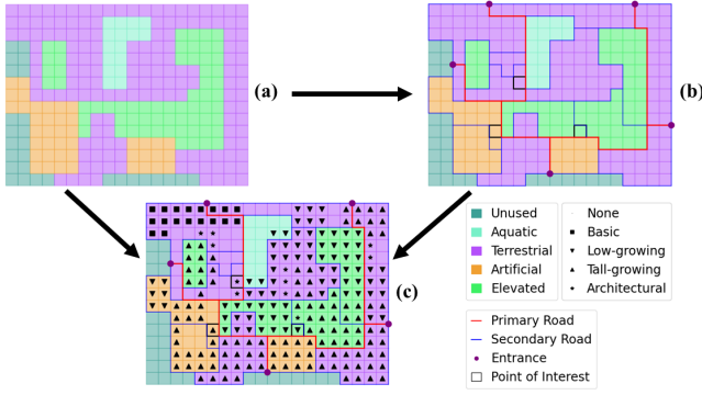
Figure 4: The results for three steps in Section 4.2. (a) The first step (Section 4.2.3) optimizes terrain types (unused, aquatic, terrestrial, artificial, and elevated) using the genetic algorithm. (b) The second step (Section 4.2.4) determines entrances, points of interest, and two-level roads connecting them. (c) The last step (Section 4.2.5) applies the genetic algorithm again to optimize the attributes (none, basic, low-growing, tall-growing, and architectural).
