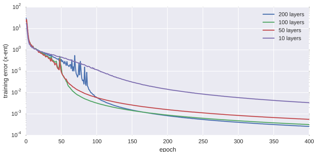
Figure 1: Training error of DVCNNs of different depth on MNIST bg-img. Even the very deep networks are able to effectively minimize the training objective without running into vanishing gradient issues. All nets were trained using the same hyperparameters.
