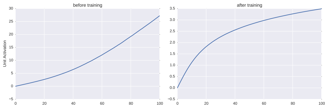
Figure 2: Average value of the non-linearity f across all units of each layers of a DVCNN using a sigmoid function with the bias set to -2 . Left: before learning has begun, Right: after the network has converged.
