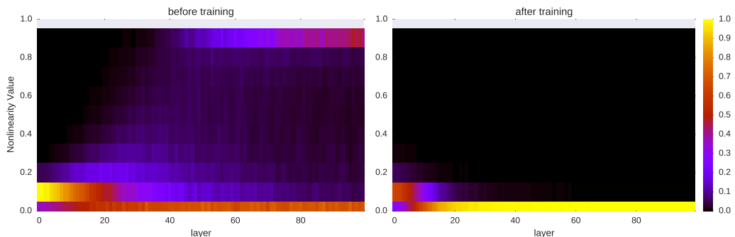
Figure 3: Distribution of the value of the non-linearity f across all units of each layers of a DVCNN using a sigmoid function with the bias set to -2 . Left: before learning has begun, Right: after the network has converged.
