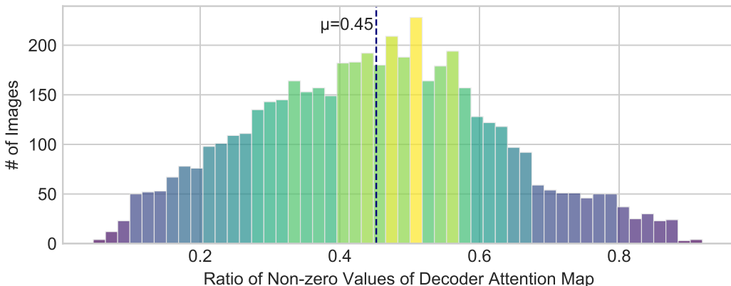
Figure 10: Distribution of the ratio of non-zero values of DAM on COCO 2017 val set.
