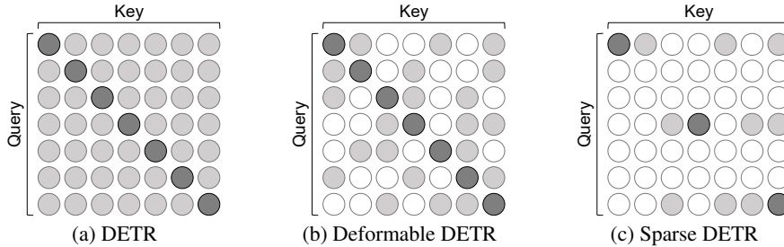
Figure 1: Attention complexity. The circles in the square matrix represent the attention between keys and queries. The gray/white circles correspond to preserved/removed connection respectively, and darker gray on the diagonal positions means where the token attends to itself. (a) Dense attention in DETR takes quadratic complexity. (b) Deformable DETR uses key sparsification, thus takes linear complexity. (c) Sparse DETR further uses query sparsification. Attention in Sparse DETR also takes linear complexity, but is much lighter than Deformable DETR’s.
