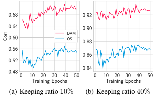
Figure 5: Correlation graph. Correlation graphs of OS and DAM during training.
