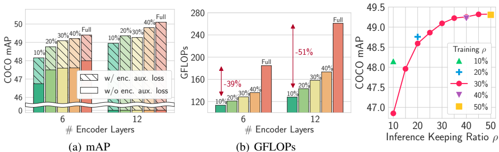
Figure 6: Ablation of # encoder layers.
