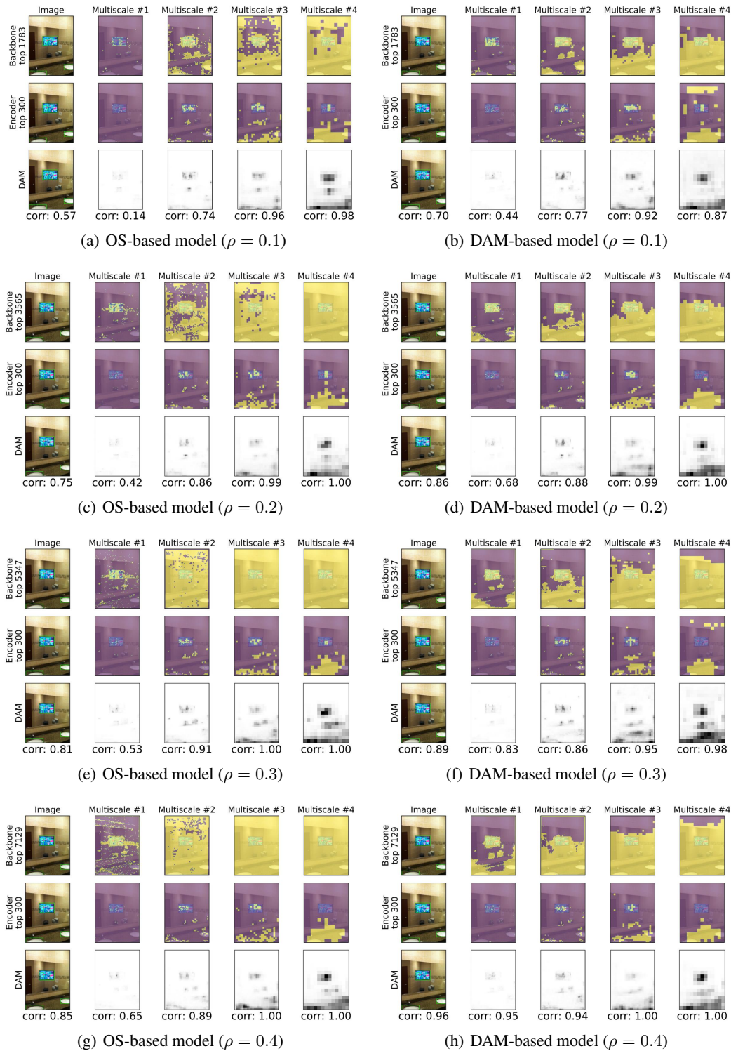
Figure 15: Visualization of selected tokens and DAM for COCO validation image #17379
