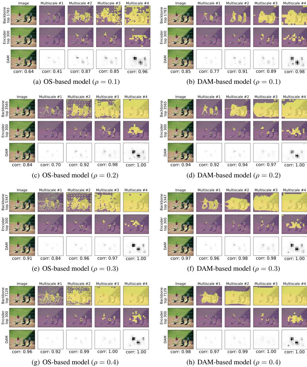
Figure 13: Visualization of selected tokens and DAM for COCO validation image #46252
