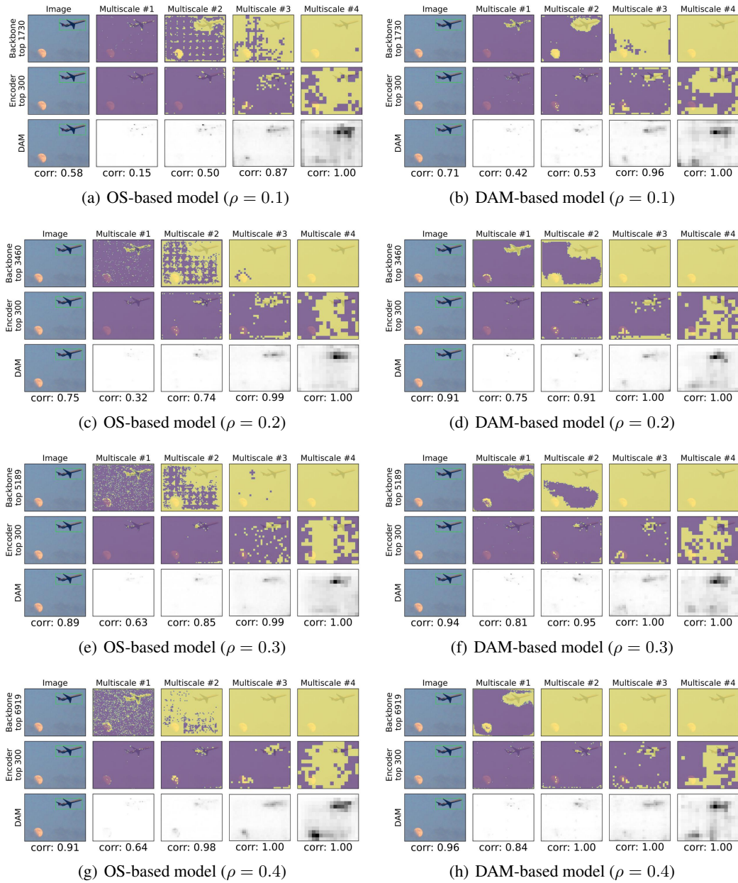
Figure 12: Visualization of selected tokens and DAM for COCO validation image #22396
