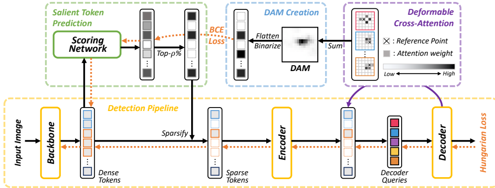
Figure 2: Illustration on how to learn a scoring network by predicting binarized Decoder cross-Attention Map (DAM), where a dashed orange arrow means a backpropagation path. The bottom box shows the forward/backward passes in Sparse DETR, and the top boxes present how to construct DAM for learning the scoring network. See Appendix A.1 for implementation details of scoring net.
