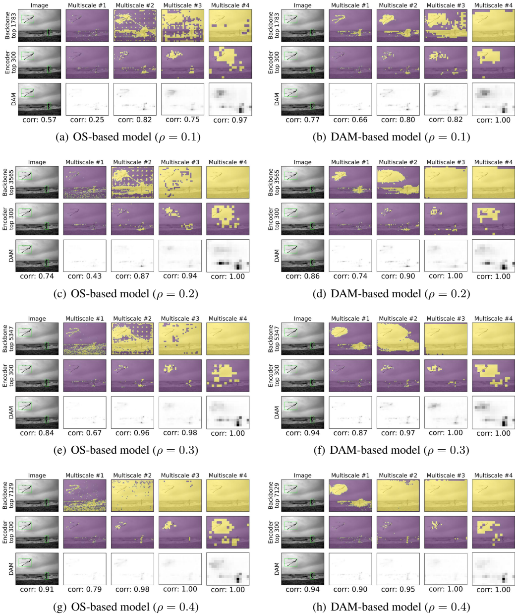
Figure 11: Visualization of selected tokens and DAM for COCO validation image #289960
