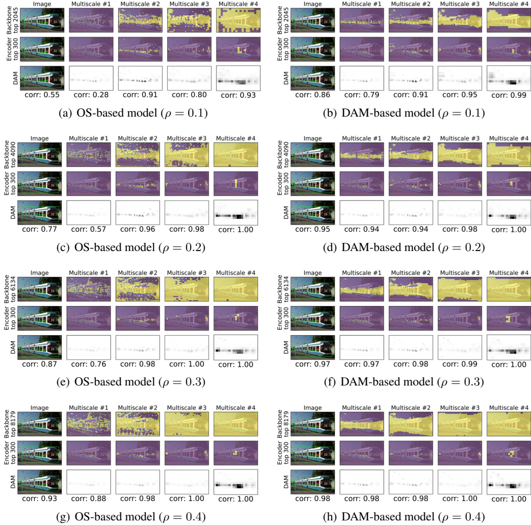
Figure 14: Visualization of selected tokens and DAM for COCO validation image #6040
