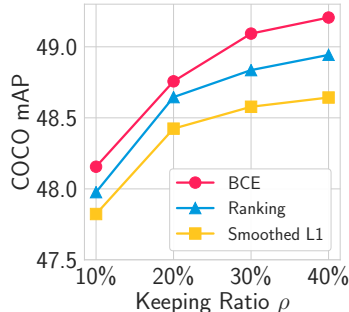
Figure 8: DAM loss ablation
