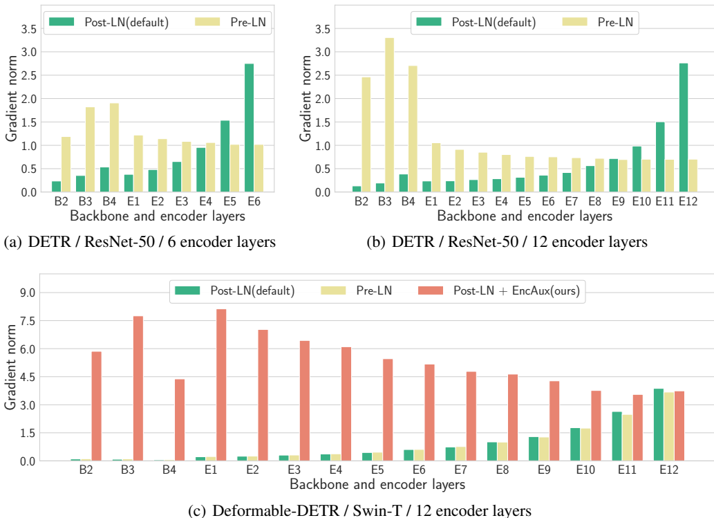
Figure 9: Layerwise gradient norm in DETR variants. An observation of the vanishing gradient problem on DETR variants with different backbones by measuring \ell^2 -norm of gradients in a layerwise manner. The first letter in x -axis label represents module name, specifically, ‘B’ for the backbone and ‘E’ for the encoder, and the second number represents i -th layer in that module. (a), (b): Layerwise gradient norm of DETR with ResNet-50 backbone. With the default settings(Post-LN), the gradient scale generally decreases as more encoder layers are stacked, while the Pre-LN technique preserves gradient magnitude even in deeper early layers. (c) : Layerwise gradient norm of Deformable-DETR with Swin-T backbone. In this case, the Pre-LN fails to prevent vanishing gradient while the encoder auxiliary loss(denoted as Post-LN + EncAux) proposed in this paper effectively resolves this issue.
