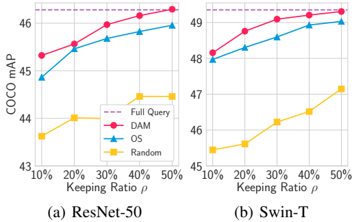
Figure 4: Selection criteria. Comparison of the performance with respect to encoder token selection criteria for different backbones.
