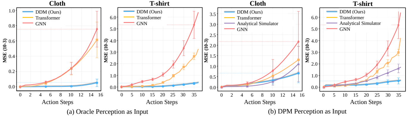
Fig. 2: Long-horizon dynamics prediction error over time. Mean Squared Error (MSE) in dynamics prediction over time under two scenarios: (a) using oracle simulation states, and (b) using DPM perception estimates, evaluated on cloths and T-shirts. Our method significantly reduces error accumulation in both cases. Error bars represent 95% confidence intervals.
