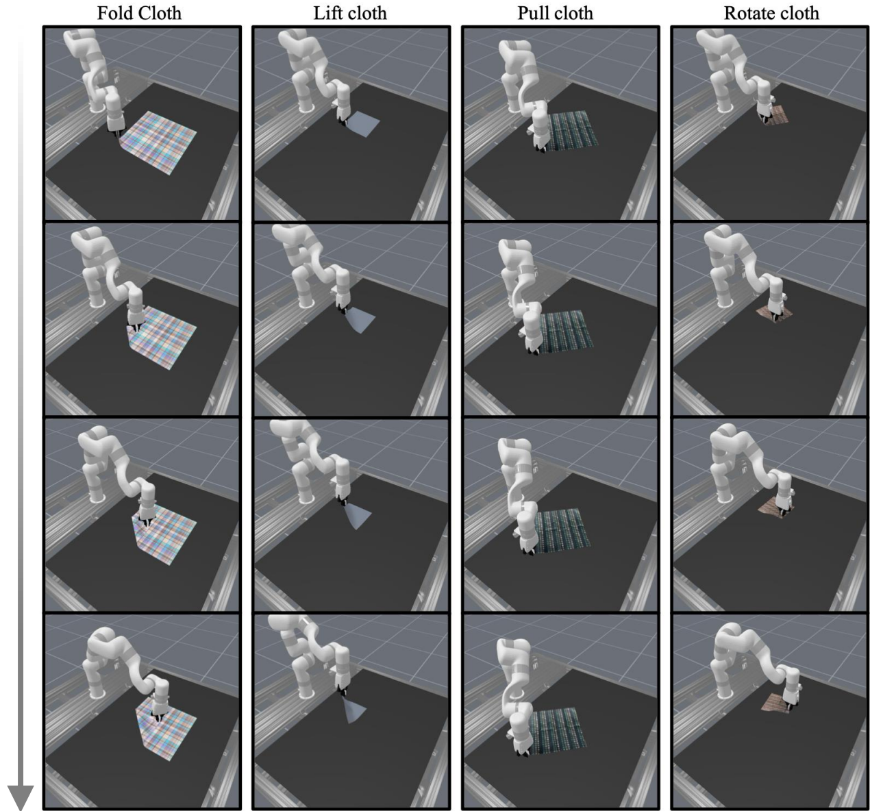
Fig. 11: Model predictive control evaluation in simulation. Demonstration of our diffusion-based dynamics model integrated with MPC across diverse manipulation tasks using xArm7, validated on various cloth types.
