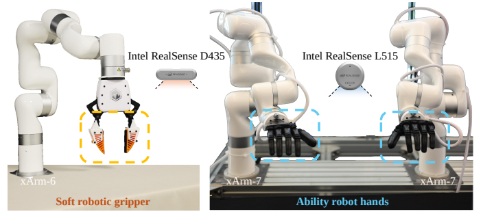
Fig. 5: Hardware overview. Our real-world platform includes a UFactory xArm-6 and a bimanual dexterous system consisting of two UFactory xArm-7 robots with Ability hands. Each robot is equipped with one RGB-D camera.
