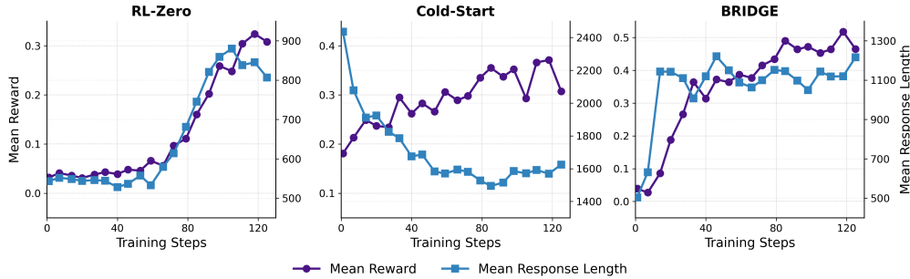
Figure 3: Training dynamics of mean reward and response length on Qwen2.5-3B.
