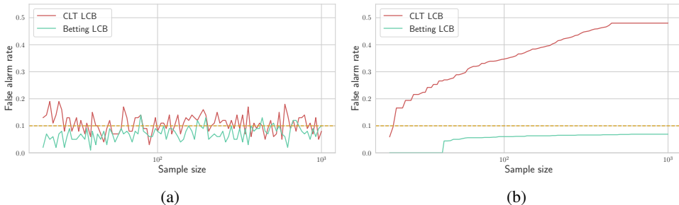
Figure 7: False alarm rate for the CLT and betting-based lower confidence bound (LCB) under: (a) fixed-time monitoring and (b) continuous monitoring. Note that both bounds control the false alarm rate at a prespecified level \delta = 0.1 under fixed-time monitoring. However under continuous monitoring, the false alarm rate of the CLT bound quickly exceeds the critical level \delta = 0.1 . At the same time, the betting LCB successfully controls the false alarm rate.
