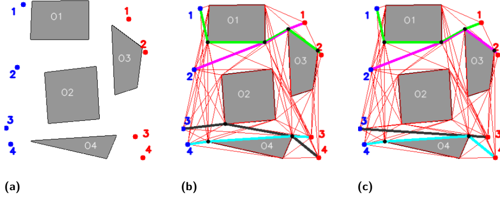
Figure 1 (a): Example of workspace W with four anchor points (in blue) and four destinations (in red). (b): Visibility graph with paths that are not solution of the NC-MAPF because the green path crosses the pink path and the black path crosses the blue path. Besides, the black path is not taut. (c): Visibility graph with paths that are solution of the NC-MAPF, even though the green and pink paths share a segment, and the black and blue paths share a vertex.
