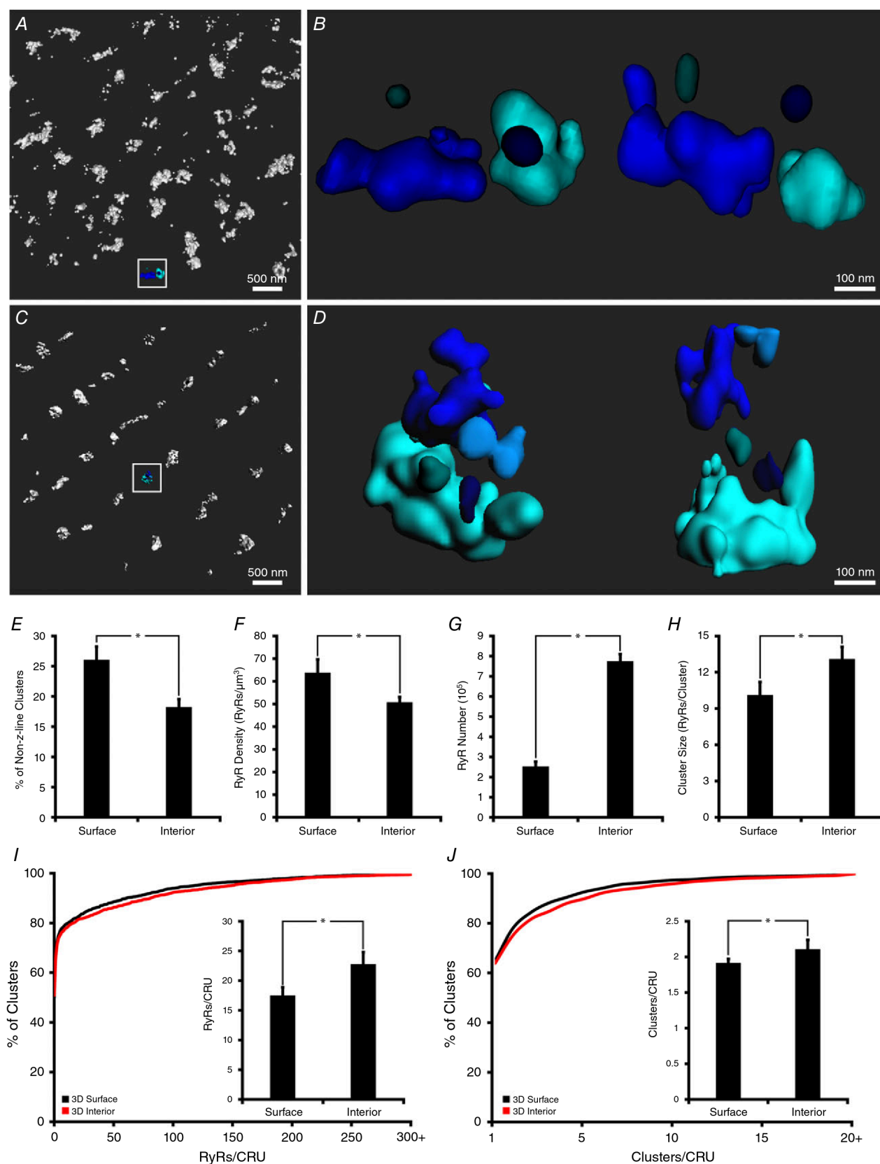
Figure 4. Comparison of 3D RyR organization at the cell surface and interior
