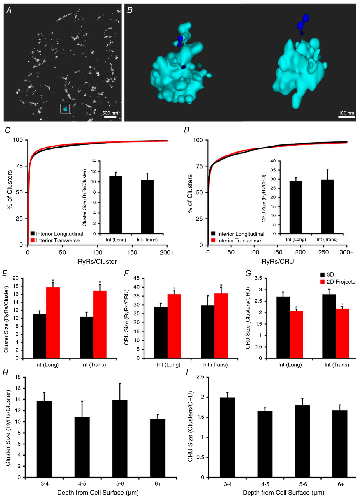
Figure 5. Comparison of 3D interior RyR cluster characteristics in longitudinally and transversely oriented cardiomyocytes
