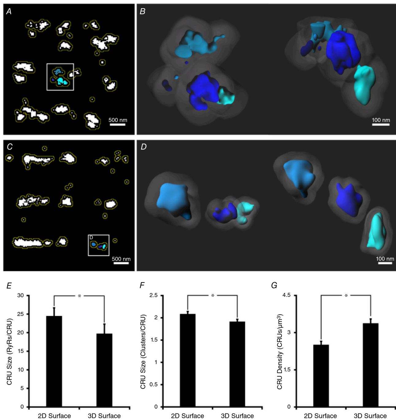
Figure 3. Quantitative comparison of cell surface \text{Ca}^{2+} release units in 2D and 3D
