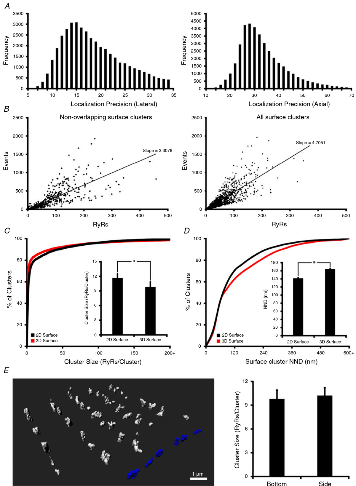
Figure 2. Quantification 3D RyR cluster characteristics at the cell surface
