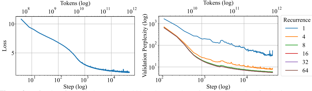
Figure 9: Left: Plot of pretrain loss over the 800B tokens on the main run. Right: Plot of val ppl at recurrent depths 1, 4, 8, 16, 32, 64. During training, the model improves in perplexity on all levels of recurrence.
