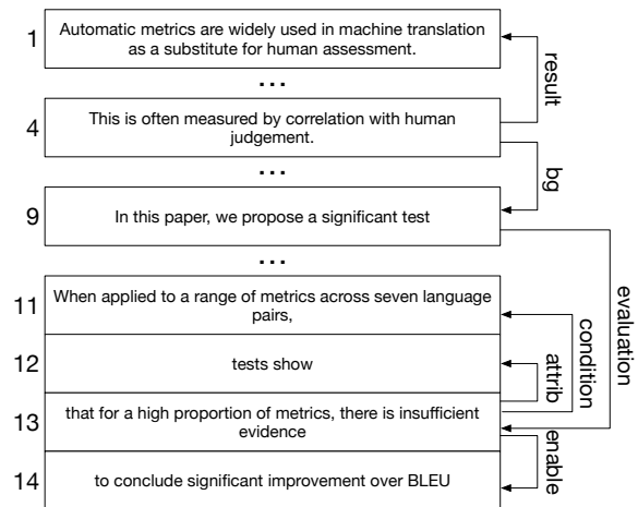
Figure 1: An excerpt discourse dependency tree in SciDTB. Each indexed block is an EDU, and the origin of the arrow pointing to a particular EDU is its head.
