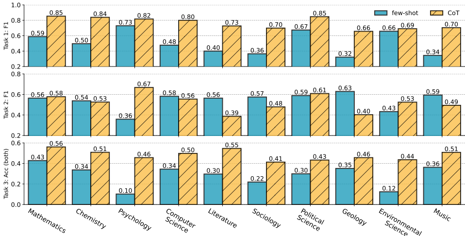
Figure 6: Performance of few-shot and Chain-of-Thought prompting divided into the other ten knowledge domains, following Figure 4.
