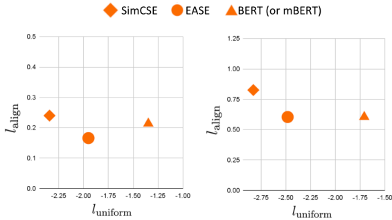
Figure 3: l_{align} - l_{uniform} plot of BERT-based (or mBERT-based) models in monolingual (left) and multilingual (right) settings.
