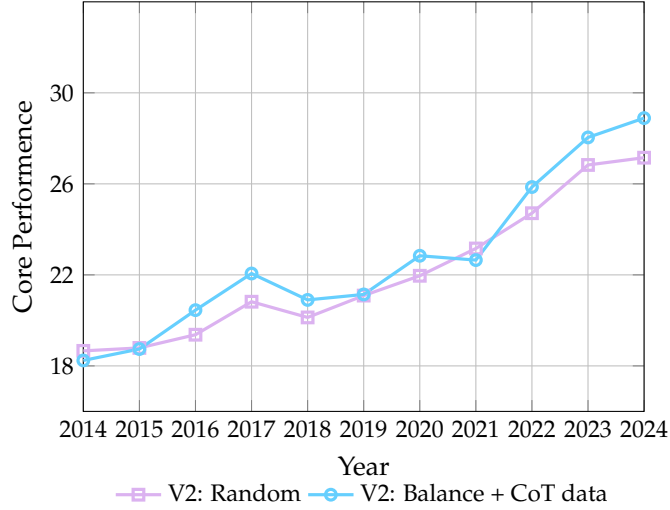
Figure 9: Ablation on fastText for each year's all dumps within 5B-token training budget
