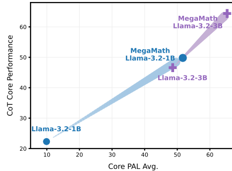
Figure 6: Training on Llama-3.2-1B/3B.
