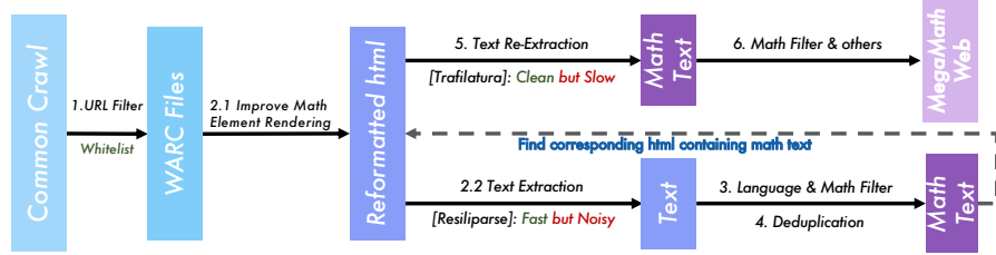
Figure 2: The pipeline for curating MegaMath-Web from Common Crawl data.
