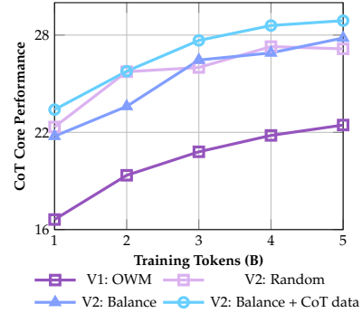
Figure 5: Ablation on fastText
