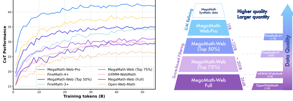
Figure 1: Comparison with existing open math corpora and MegaMath-Web subsets.
