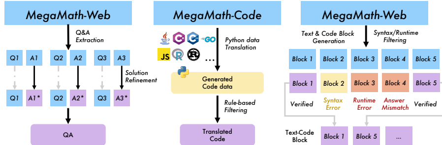
Figure 4: The pipeline for curating synthetic data. Left: QA data generation; Middle: Python code augmentation; Right: text & code block data curation.
