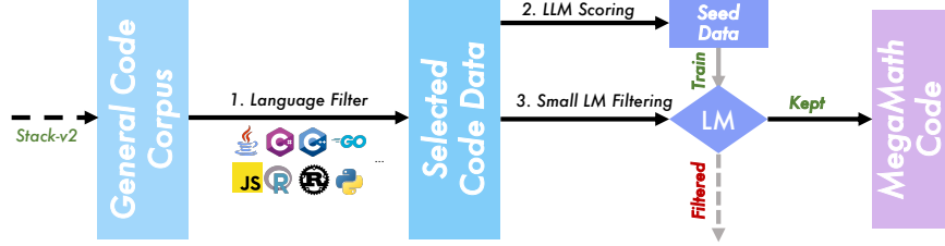
Figure 3: The pipeline for curating MegaMath-Code.
