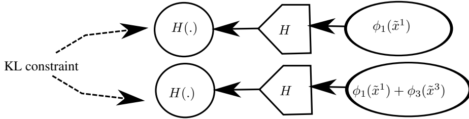
Figure 2: The MV-BiGAN additional components. In this example, we consider a case where only \tilde{x}^1 is available (top level) and a second case where both \tilde{x}^1 and \tilde{x}^3 are available. The distribution P(z|\tilde{x}^1, \tilde{x}^3) is encouraged to be "included" in P(z|\tilde{x}^1) by the KL constraint. The aggregation of the views is made by the \phi_k functions that are learned conjointly with the rest of the model.
