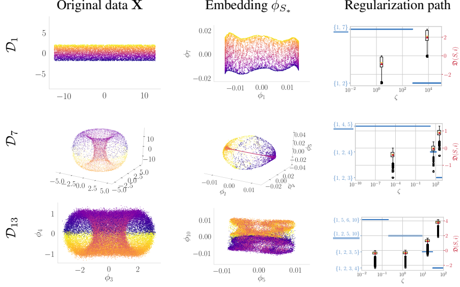
Figure 2: Experimental result for synthetic datasets. Rows correspond to different synthetic datasets (please refer to Table S2). Optimal subset S_* is selected by INDEIGENSEARCH.
