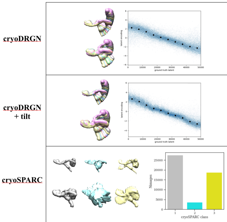
Figure S10: Reconstruction results for the linear 1D dataset by cryoDRGN and by discrete multiclass reconstruction in cryoSPARC. Top : Reconstructed structures from cryoDRGN sampled along the latent space (at depicted points) matches the ground truth variation. The predicted latent encoding correlates with the ground truth latent degree of freedom. Middle : CryoDRGN results with tilt series. Bottom : Reconstructed volumes and the distribution of images over clusters from discrete multiclass reconstruction in cryoSPARC. Volumes are visualized at high and low isosurface, showing artifacts in the cryoSPARC structures.
