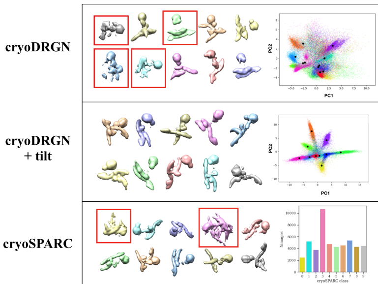
Figure S13: Reconstruction results for the dataset containing 10 discrete structures by cryoDRGN and by discrete multiclass reconstruction in cryoSPARC. Top : The majority of reconstructed structures from cryoDRGN sampled along the latent space (at depicted points) matches the ground truth structures, however some are incorrect (red boxes), and the learned data manifold is not well separated into clusters. Middle : CryoDRGN results with tilt series reconstructs the 10 structures and clusters the images in the latent space accordingly. Bottom : Reconstructed volumes from discrete multiclass reconstruction in cryoSPARC and the distribution of images over clusters. CryoSPARC learns 8 out of 10 structures correctly.
