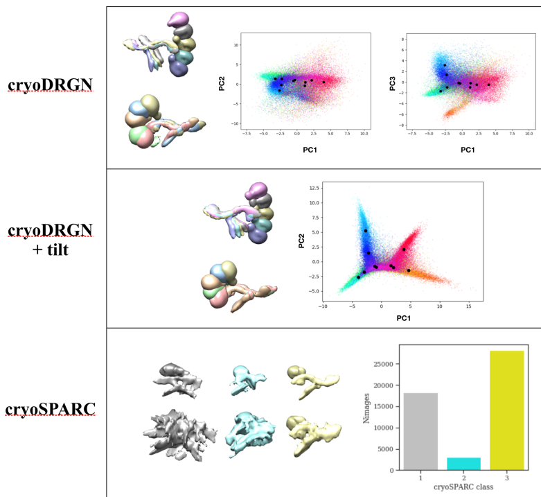
Figure S12: Reconstruction results for the linear 2D dataset by cryoDRGN and by discrete multiclass reconstruction in cryoSPARC. Top : Reconstructed structures from cryoDRGN sampled along the latent space (at depicted points) roughly matches the ground truth variation, however the distribution of images in the latent space does not recapitulate the true data manifold well. Middle : CryoDRGN results with tilt series reconstructs the true structural variation and the distribution of images in the latent space matches the topology of the true data manifold. Bottom : Reconstructed volumes and the distribution of images over clusters from discrete multiclass reconstruction in cryoSPARC. CryoSPARC volumes are visualized at high and low isosurface, showing artifacts at low isosurface
