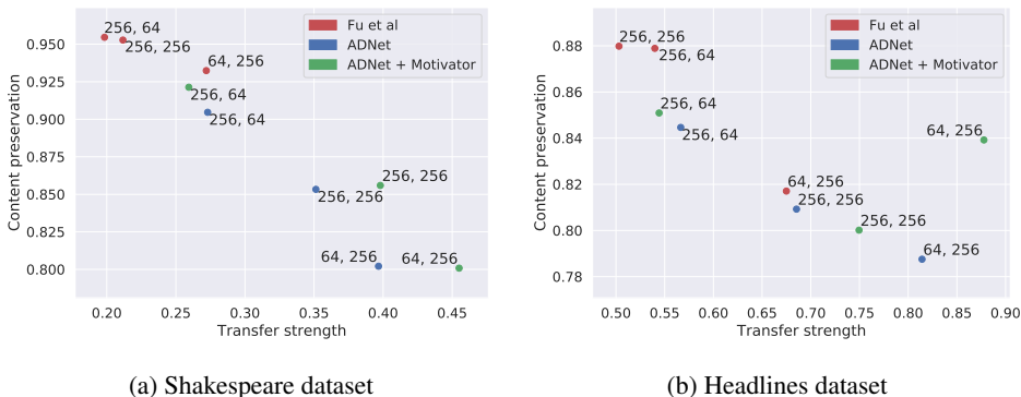
Figure 2: Transfer strength vs Content preservation (see subsection 5.1) for different combination of the size of the meaning and form vectors. Each point is labeled with ‘‘m; f’’ meaning vector size, f form vector size.’’
