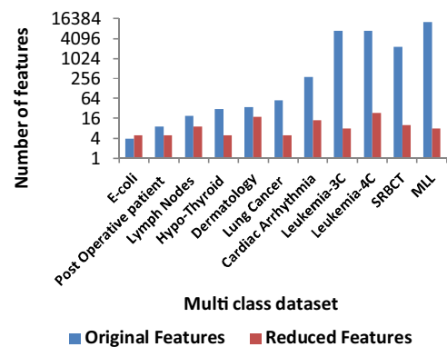
Fig. 4. SVEGA Performance on Multi Class Data.
