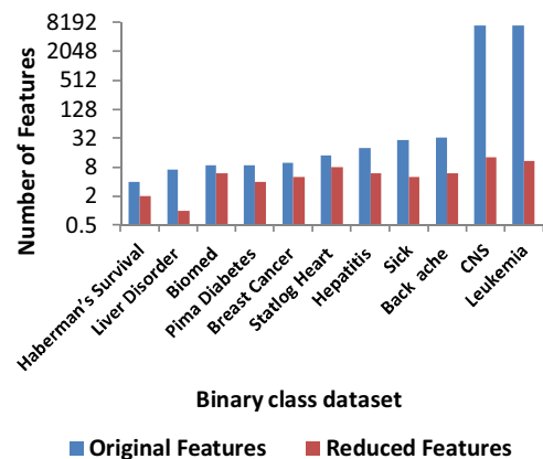
Fig. 3. SVEGA Performance on Binary Class Data.
