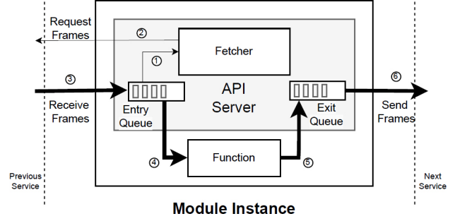
Fig. 6: Module instance in pseudo-central queue design.
