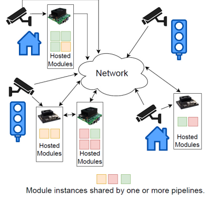
Fig. 4: Overview of distributed edge devices featuring multiple VA pipelines. Each colored box represents a VA module hosted on the edge device. The modules are replicated as needed.
