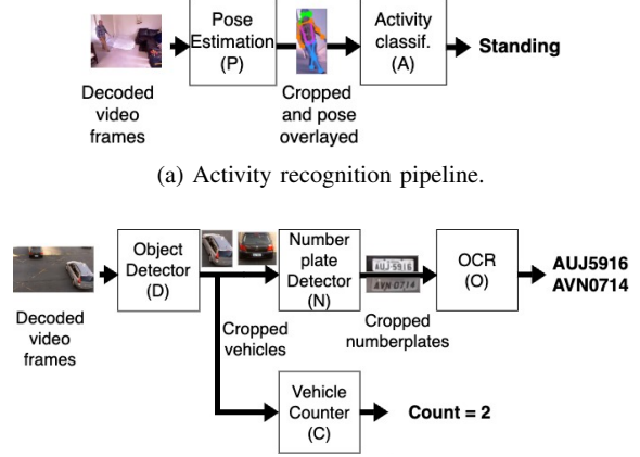
(b) Number plate recognition and vehicle counting pipelines; object detector is a common function for these two pipelines.
