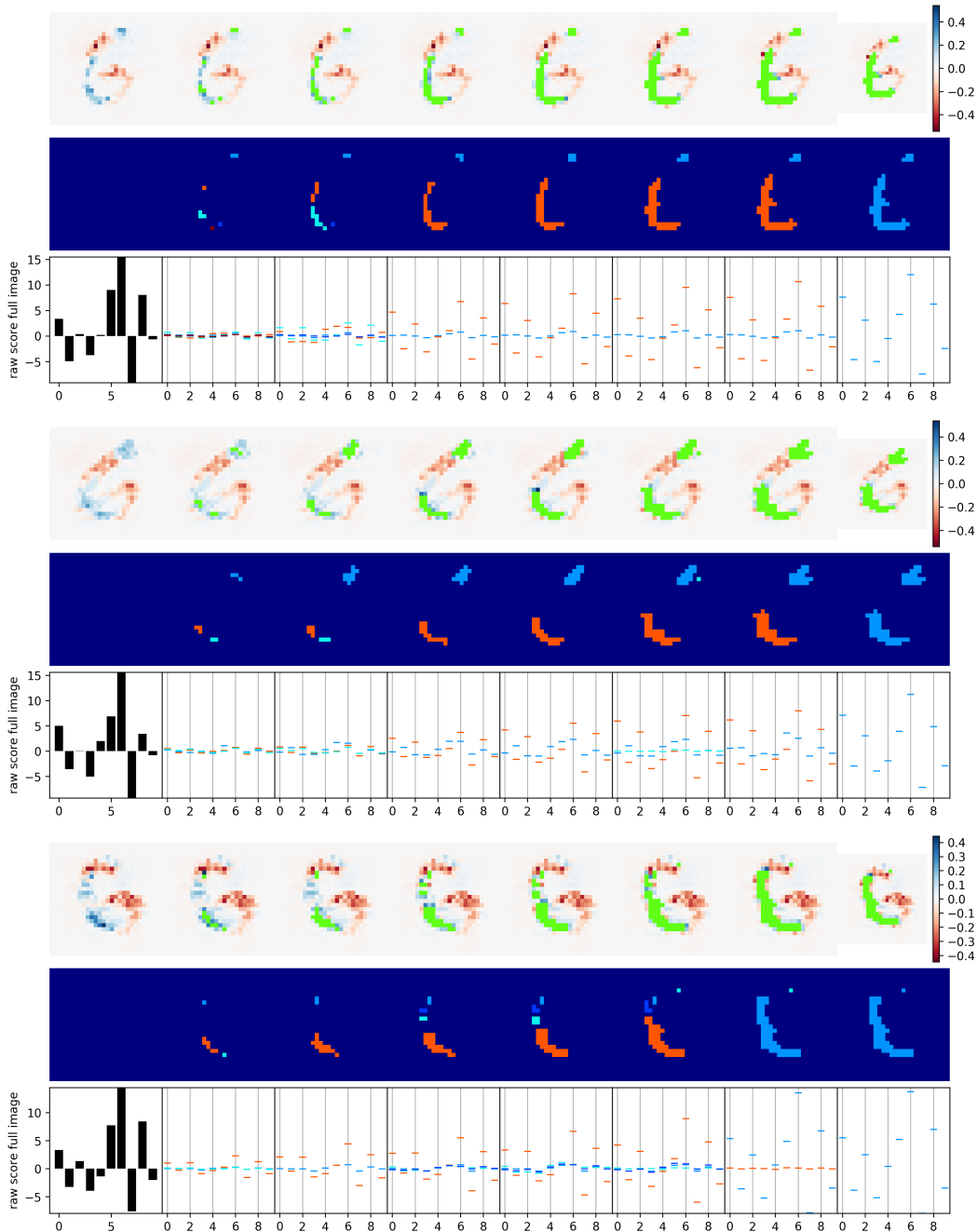
MNIST top-predicted examples. Here, the model used is the same as in Sec 4.3.2 and the interpretation of the figure produced is the same as in Fig 3.
