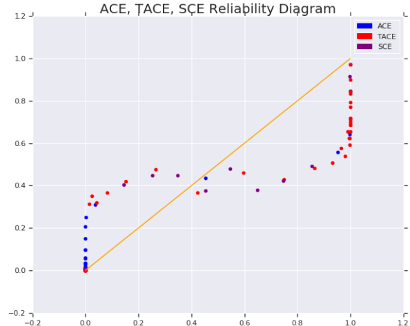
Figure 2: Reliability Diagram over adaptive metrics for a CNN on Fashion-MNIST validation data. TACE and ACE with 100 bins, SCE with 10.
