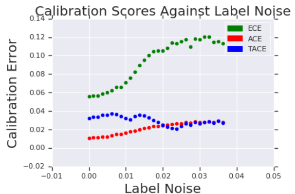
Figure 8: As label noise increases, ECE is outperformed by ACE and TACE. This shows that ECE becomes a worse approximation of true calibration error as class predictions beyond the predicted one matter more. (The x = 0 extreme has a true data distribution with deterministic y ; x \rightarrow \infty extreme has a true data distribution with uniform y .)
