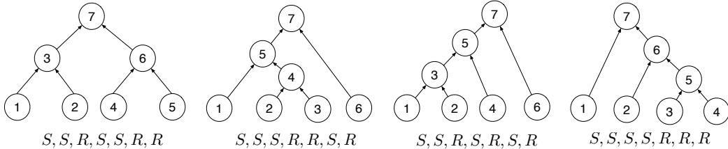
Figure 1: Four examples of trees and their corresponding SHIFT (S) and REDUCE (R) sequences. In each of the examples, there are 4 input words (4 leaf nodes), so 7 operations (4 S, 3 R) are needed to construct a valid tree. The nodes are labeled with the timesteps in which they are introduced to the trees t \in \{1, \dots, 7\} . A SHIFT operation introduces a leaf node, whereas a REDUCE operation introduces a non-leaf node by combining two previously introduced nodes. We can see that different S-R sequences lead to different tree structures.
