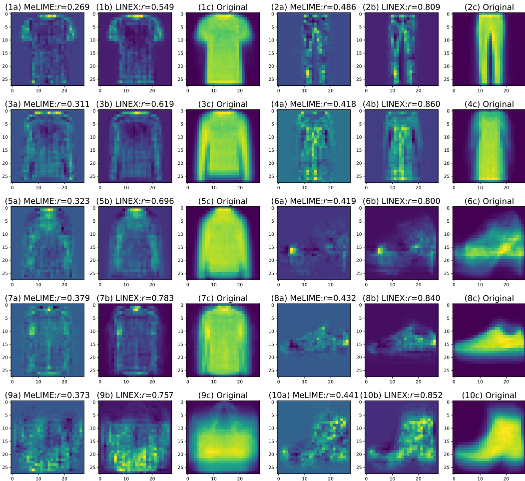
Figure 21: Results using realistic perturbations for FMNIST dataset with mean feature importances for all classes:1-10 ( T-shirt/top , Trouser , Pullover , Dress , Coat , Sandal , Shirt , Sneaker , Bag and Ankle boot ). (a) Mean feature attributions of all images in the class using MeLIME. (b) Mean feature attributions of all images in the class using LINEX. (c) Mean of all images in the class. The r values show Pearson’s correlation between average feature attributions and mean of the original images from the respective classes. We observe that LINEX explanations/attribution exhibit significantly higher correlation with the original images belonging to a particular class (i.e. high CAC).
