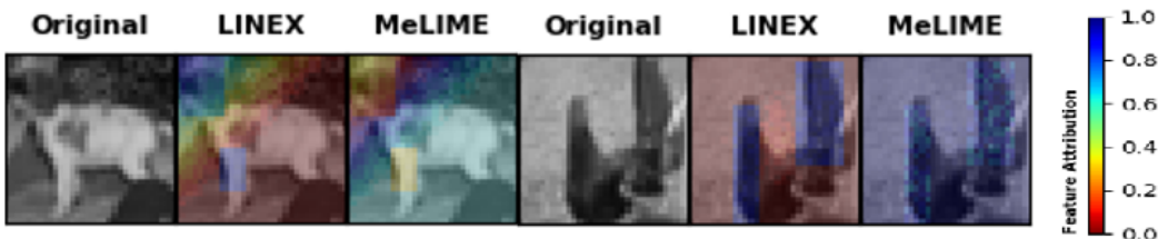
Figure 3: Sample results using CIFAR10 dataset for dog and bird class. As can be seen LINEX focuses more on salient features such as head and legs for the dog, and wings for the bird (rather than also the background). More examples are shown in Appendix G.
