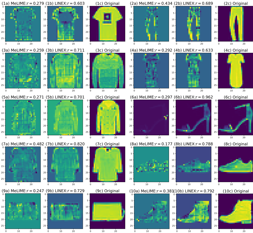
Figure 20: Results using individual samples for realistic perturbations for FMNIST dataset for all classes: 1-10 ( T-shirt/top, Trouser, Pullover, Dress, Coat, Sandal, Shirt, Sneaker, Bag and Ankle boot ). (a) MeLIME feature attributions for an image. (b) LINEX feature attributions for an image. (c) Original image in the class. The r values show Pearson’s correlation between feature attributions and the original image from the respective class. We observe that LINEX attributions/explanations exhibit significantly higher correlation with the original image belonging to a particular class (i.e. high CAC).
