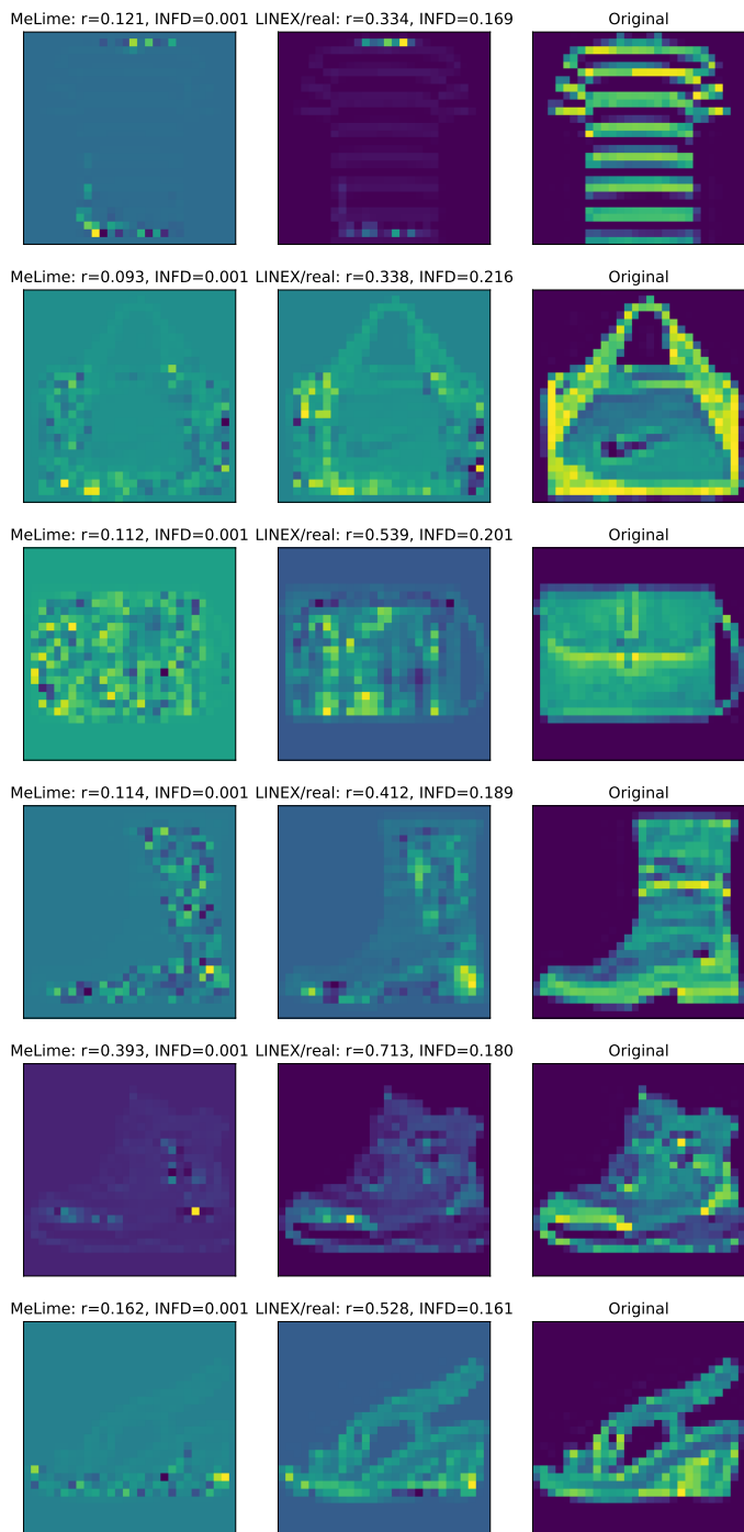
Figure 23: Error analysis for a chosen set of examples in FMNIST using MeLIME and LINEX/real methods. The three columns are the MeLIME feature attributions, LINEX/real feature attributions, and the original images. The rows correspond to different examples. We show the Pearson’s correlation coefficient between feature attributions and mean of the original images from the respective classes ( r ) and instance-level infidelity (INFD) measures. LINEX seems to highlight important features like stripes in the t-shirt, handles of the bags, outlines of the boots/shoes more prominently, while MeLIME seems to overfit to the data while missing out on highlighting some key features prominently.
