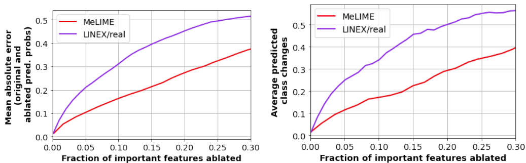
Figure 25: Ablation analysis to determine if the features deemed important by the explanation methods are actually considered important for prediction by the black box model. We see that features chosen by LINEX impact the prediction of the black box model much more than those chosen by MeLIME. This is true with respect to both MAE measure (left) between the predicted probabilities before and after ablation for winning (or argmax) class, and the change in predicted classes (right) before and after ablation. Higher values here mean that the features chosen by the explanations are more relevant for the black box to make its predictions. The maximum value of both measures is 1.0.
