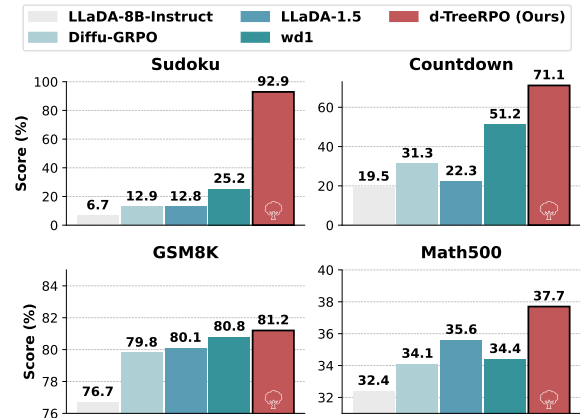
Figure 1: Performance comparison of d -TreeRPO with existing dLLM RL methods on four reasoning benchmarks, using LLaDA-8B-Instruct as base model.
