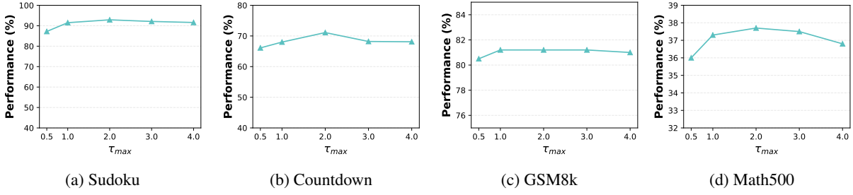
Figure 12: Evaluation performance under different \tau_{max} settings on the four evaluated tasks.
