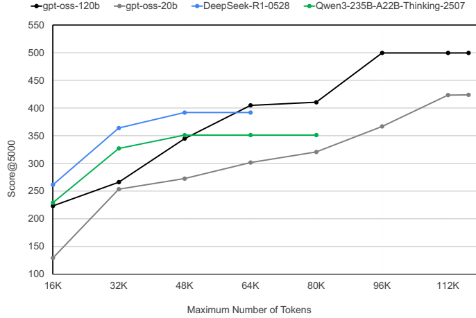
Figure 7: Score@K for different maximum number of tokens in generation with different models.
