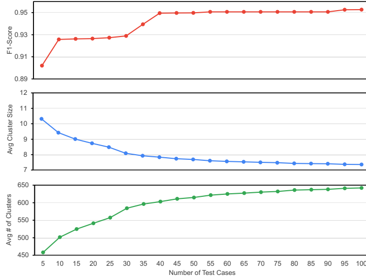
Figure 4: Shown are the cluster purity (F1-score), average cluster size, and average number of clusters for different numbers of test cases. Results are reported for K = 5000 using gpt-oss-120b .
