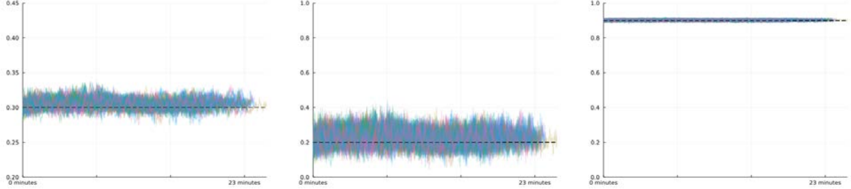
Figure 9: Robustness Comparison on First-order RBC: Trace Plot
