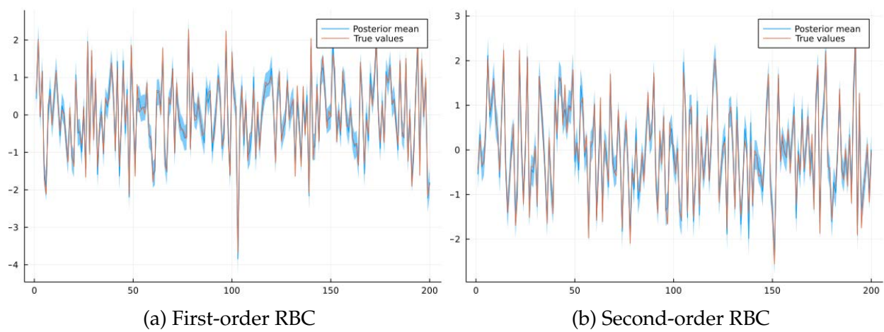
Figure 6: Inferred TFP Shocks of RBC Model
