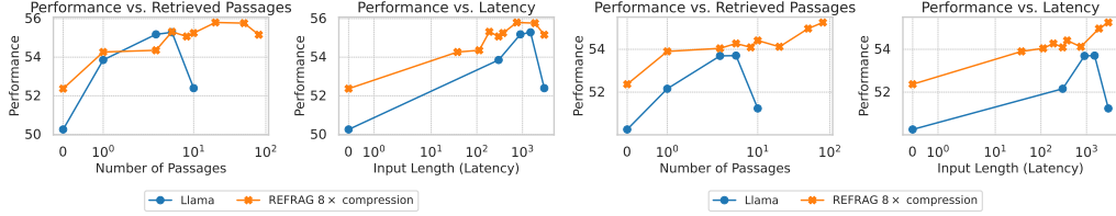
Figure 4: RAG performance comparison under a strong retriever scenario (left) and a weak retriever scenario (right). REFRAG perform similarly to LLaMA model under the same retrieved passages (slightly better in a weaker retriever case) while outperform significantly under the same latency.
