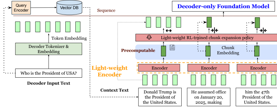
Figure 1: The main design of REFRAG. The input context is chunked and processed by the light-weight encoder to produce chunk embeddings, which are precomputable for efficient reuse. A light-weight RL policy decide few chunks to expand. These chunk embeddings along with the token embeddings of the question input are fed to the decoder.
