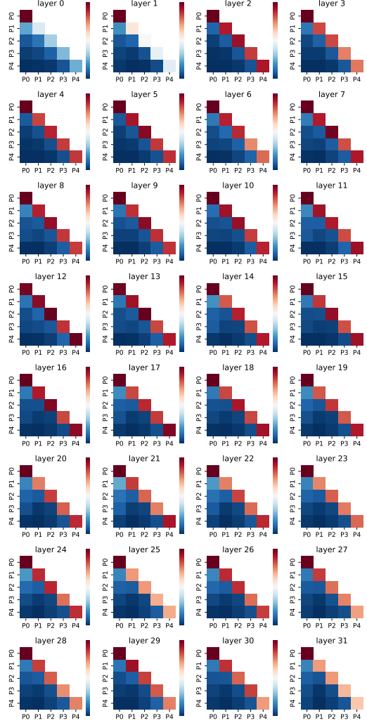
Figure 7: Attention value visualization for different retrieved passages for different layers for LLaMA-2-7B-Chat model. The diagonal values are the averaged attention value for tokens within each passage while the off-diagonal values are the averaged attention value between tokens from different passages. The detail of retrieved passages is in Table 10.
