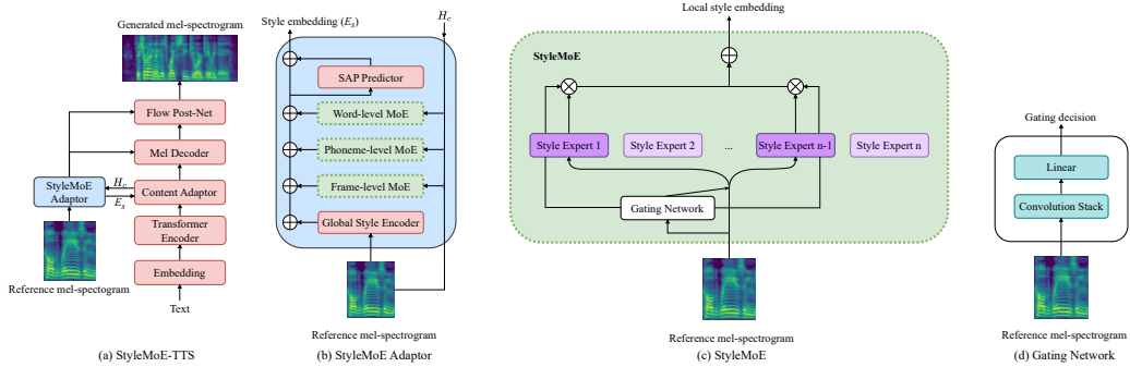
Figure 1: The architecture of StyleMoE-TTS. Red modules represent modules from GenerSpeech (15). Green modules represent the Mixture of Experts layer. Purple modules represent style experts. The darker purple modules represent the style experts chosen by the gating network. Subfigures (a) and (b) illustrate the integration of StyleMoE into StyleMoE-TTS. Subfigure (c) depicts the StyleMoE layer, wherein each style expert block is a style reference encoder. Subfigure (d) illustrates the gating network.
