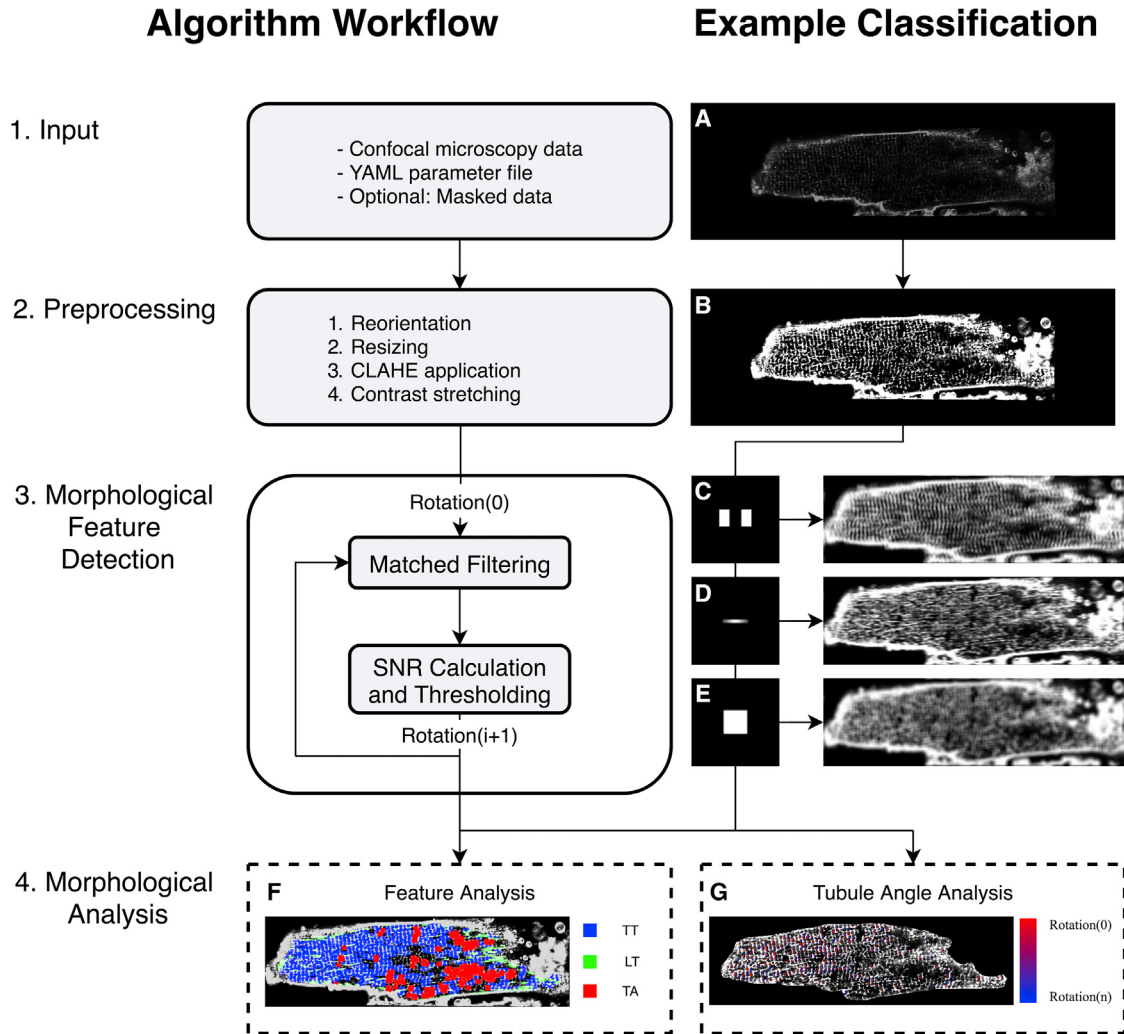
FIGURE 1 Unicellular matched-filtering protocol: 1) input of confocal microscopy data, YAML (.yaml) parameter file, and optional user generated mask for that data, for which (A) shows sample input image. YAML parameter file construction is explained in Supporting Materials and Methods , Section S1.4; 2) integrated preprocessing routines in which (B) shows sample preprocessed image; 3) morphological feature detection via matched filtering and signal/noise ratio calculation. (C–E) Matched filters and sample signal/noise ratio calculation via convolution for TT, LT, and TA filters, respectively; 4) morphological analysis of features, feature density, and feature rotation. (F) Sample morphological feature content analysis exhibiting high TT content relative to other morphological features. (G) Sample tubule striation angle analysis with high angle variance. To see this figure in color, go online.
