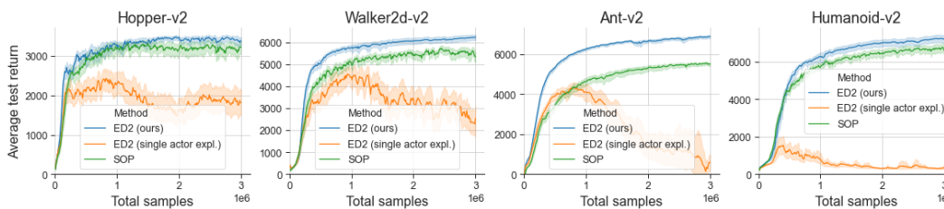
Figure 34: The average test returns across the training of ED2, ED2 with the single actor for exploration, and the baseline.
