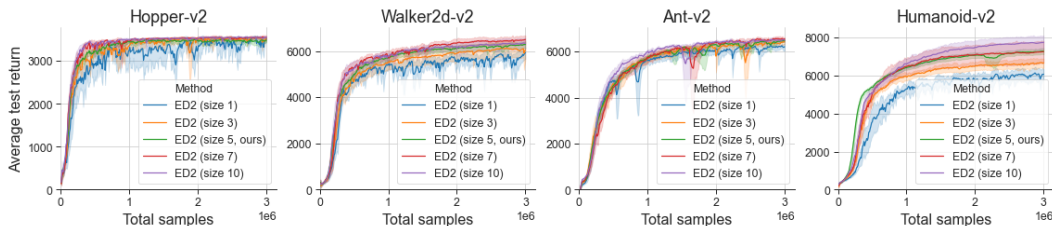
Figure 17: The average test returns across the training of ED2 with a different number of actor-critics.
