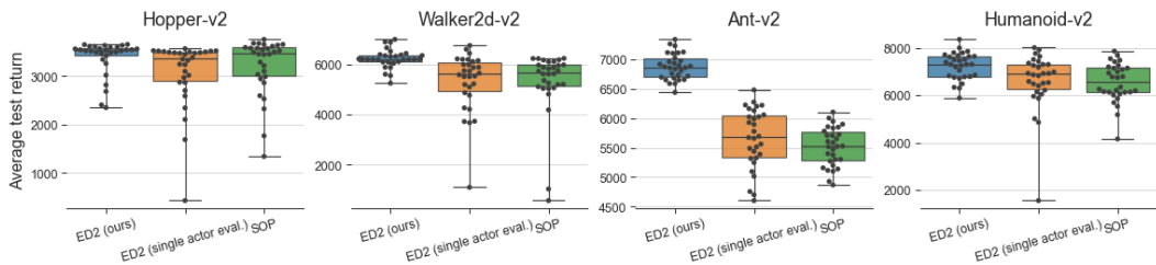
Figure 32: The dots are the average test returns after training ( 3M samples) of each seed of ED2, ED2 with the single actor for exploitation, and the baseline. The distance between each box's top and bottom edges is the interquartile range (IQR). The whiskers spread across all values.
