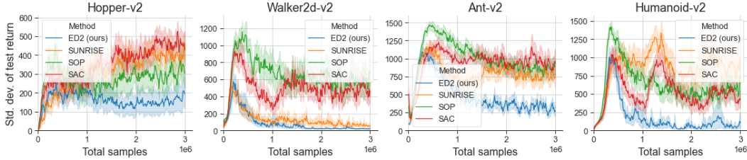
Figure 3: The standard deviation of test returns across training (lower is better), see Section 2.
