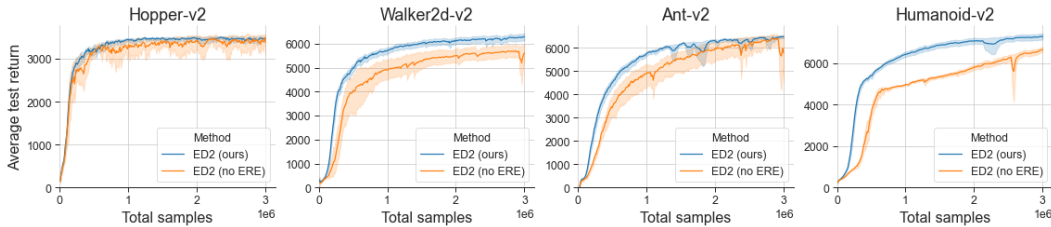
Figure 36: The average test returns across the training of ED2 with and without the ERE replay buffer.
