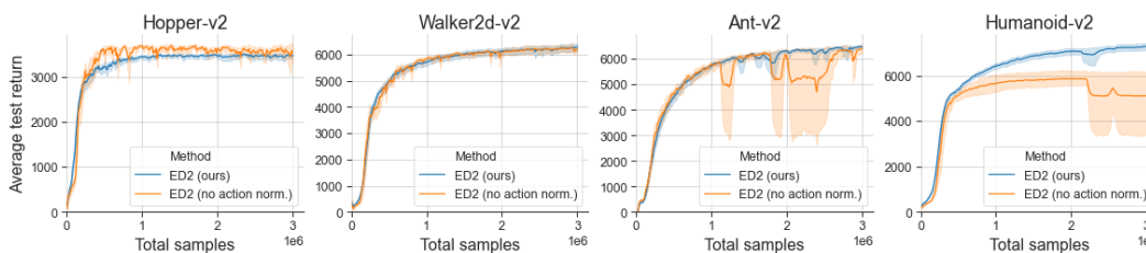
Figure 35: The average test returns across the training of ED2 with and without the action normalization.
