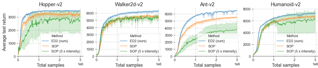
Figure 20: The average test returns across the training of ED2 and SOP with one or five updates for every step in an environment.
