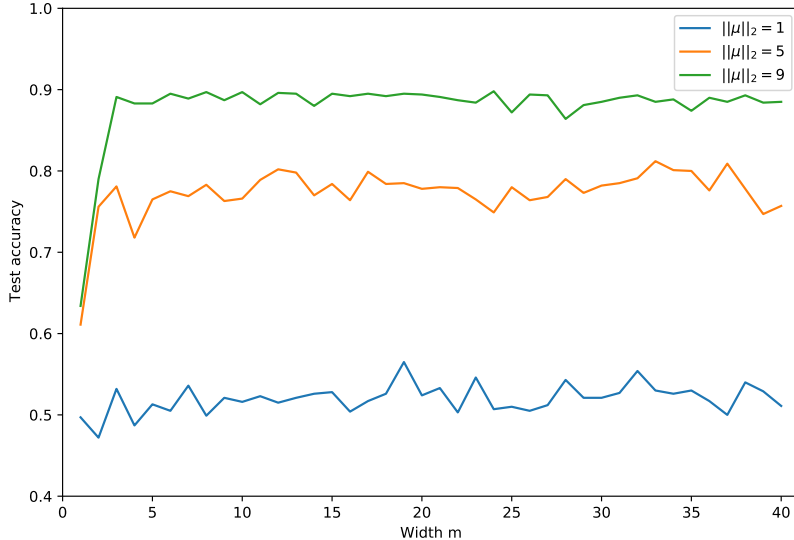
Figure 3: Test accuracy of neural networks with different widths m under different signal strengths. The x -axis represents the value of width m ranging from 1 to 40, whereas the y -axis is the test accuracy. The different lines on the plot represent the test accuracy achieved under different norms of \|\mu\|_2 .
