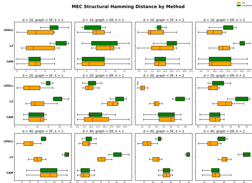
Figure 12: Structural Hamming distance (SHD) between Markov equivalence classes (MEC) of recovered and ground truth graphs. LOGLL (i.e. LOGLL-NOTEARS) stands for NOTEARS method with log-likelihood and quasi-MCP, L2 (i.e. NOTEARS) stands for NOTEARS method with least square and \ell_1 .
