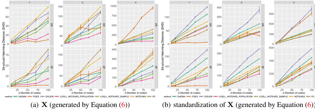
Figure 1: Results in terms of SHD between MECs of estimated graph and ground truth. Lower is better. Column: k = \{1, 2, 4\} . Row: random graph types. \{ER, SF\} - k = \{Scale\text{-Free}, Erd\acute{o}s\text{-R\'{e}nyi}\} graphs with kd expected edges. Here p = \{10, 20, 50, 70, 100\} , n = 1000 .
