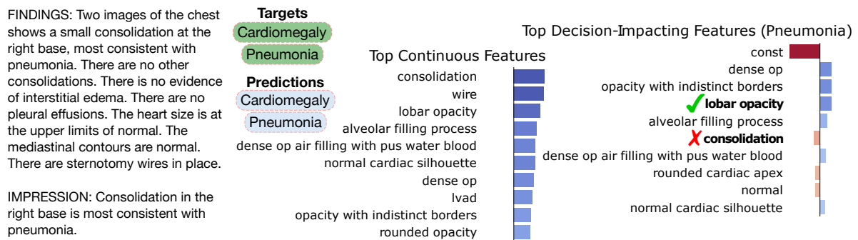
Figure C.2: Qualitative Example of Features and Feature Influence for Pneumonia. (Similar to Figure 7.) This seems to correctly predict Pneumonia, but this happens in spite of consolidation being incorrectly identified by the linear model as not supporting Pneumonia. These plots make clear that this is not a mistake of the feature extractor at inference time because consolidation is among the top Features. The mistake comes from the linear model having a negative coefficient for consolidation.
