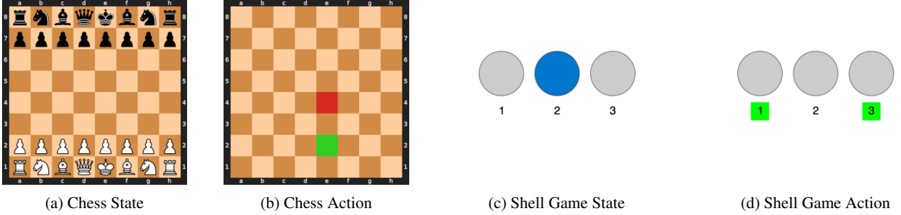
Figure 1: Illustration of the two domains used in this work. (a) An example Chess board state. (b) The chess move (action) rendered as an image. (c) An initial shell game state with the blue ball under a shell. (d) Image action representing shells at positions one and three being swapped.
