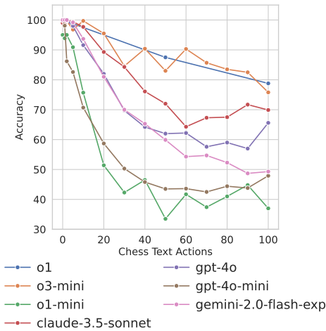
(a) Chess zero-shot accuracy with text actions.
