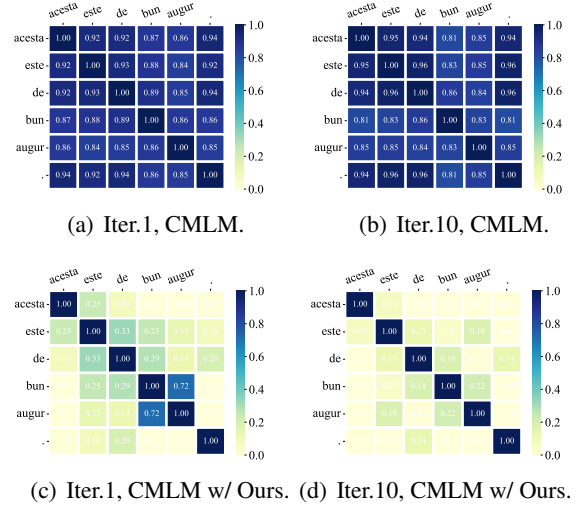
Figure 4: Token cosine similarity matrix of CMLM w/o and w/ our methods in iteration 1/10 on distill WMT16 EN→RO dataset.
