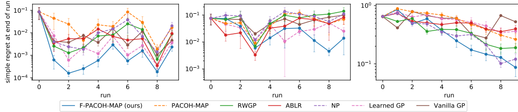
Figure 6: Lifelong BO performance on two simulated function environments and one hyper-parameter tuning benchmark (RPart). The reported results are averages over seeds and random sequences of tasks alongside 95% confidence intervals. While other meta-learners struggle to achieve positive transfer, F-PACOH is able to significantly improve the BO performance as it gathers more experience.
