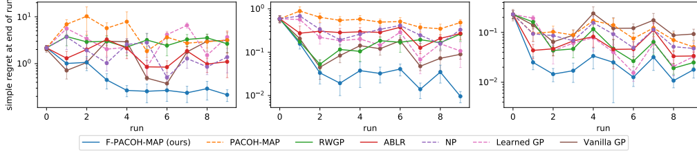
Figure 4: Lifelong BO performance on two simulated function environments and one hyper-parameter tuning benchmark (RPart). While other meta-learners struggle to achieve positive transfer, F-PACOH is able to significantly improve the BO performance as it gathers more experience.
