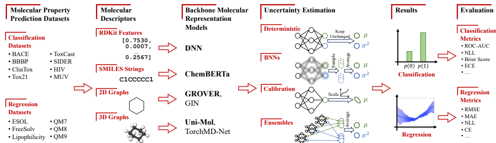
Figure 1: MUBEN overview with datasets, backbones, UQ methods and metrics enumerated.
