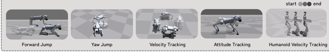
Figure 3: Open-Loop Locomotion Tasks: Forward Jump : Jump forward to a predefined distance of 0.85m. Yaw Jump : Jump and do Yaw Rotation to a predefined yaw angle of 135 degrees. Velocity Tracking : Track a sequence of Open loop 2D twist commands, Attitude Tracking : Track a sequence of roll and pitch commands, Humanoid Velocity Tracking : Track a sequence of 2D twist velocity commands for a humanoid.
