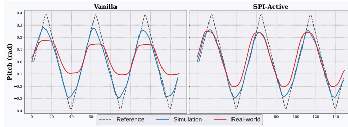
Figure 4: Comparison between SPI-Active and Vanilla policies in both simulation and real-world execution. SPI-Active yields a closer match to simulation, suggesting improved sim-to-real consistency.
