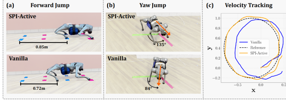
Figure 5: Task Performance comparison of SPI-Active vs Vanilla in (i) Forward Jump, (ii) Yaw Jump, (iii) and Velocity Tracking
