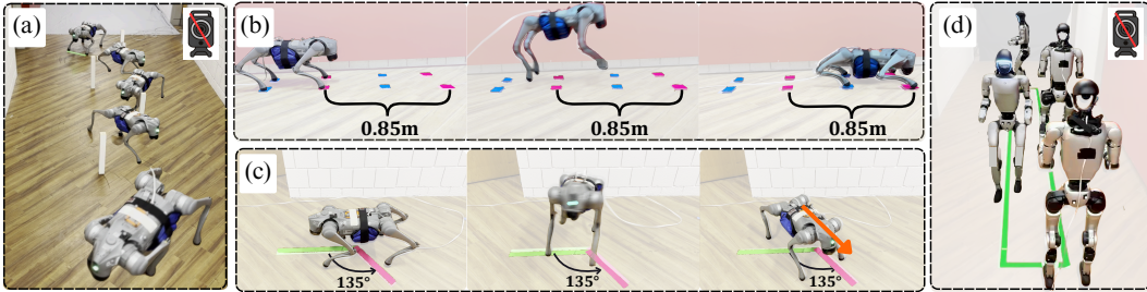
Figure 1: SPI-Active enables high-fidelity Sim-to-Real transfer across diverse locomotion tasks. To highlight the precision, all tasks are open-loop tracking without global position feedback . (a) High-Speed Weave Pole Navigation, (b) Precise Forward Jump, (c) Precise Yaw Jump, and (d) Humanoid Precise Velocity Tracking.
