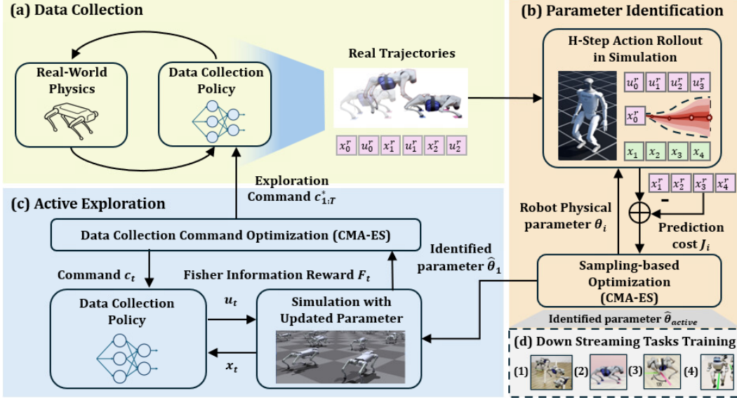
Figure 2: Overview of SPI-Active . Data Collection : Collect real-world trajectories using RL policies or motion priors. Parameter Identification : Estimate physical parameters via simulation-to-real rollout matching by sampling-based optimization. Active Exploration : Optimize input commands of a multi-behavioral policy to maximize Fisher Information and gather informative data. Downstream Task Training : Use identified parameters to train accurate locomotion controllers.
