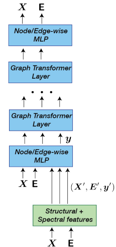
Figure 5: Architecture of the denoising
