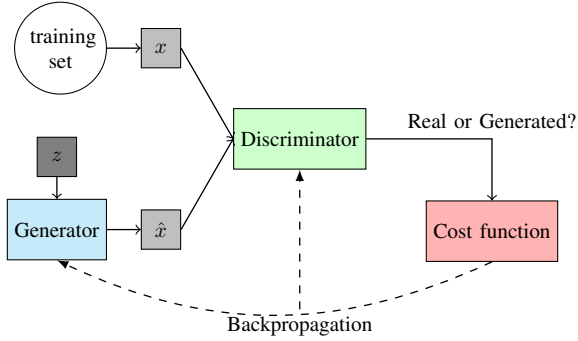
Figure 15. Generative Adversarial Networks Framework.
