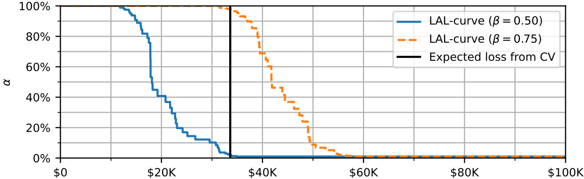
Figure 1: Model error diagnostic. Consider a predictive model f(X) of house price Y in an area described by a feature vector X . How will this model perform in m future price predictions? We evaluate the model using the prediction error \ell(X, Y) = |Y - f(X)| as the chosen loss function. The cross-validation method (CV) evaluates the model by estimating the expected out-of-sample loss, which in this case is circa $36K (indicated by black vertical line). Being an estimate of an expectation, it provides limited information about what individual loss values might be observed. Suppose the model will be used in m = 100 prediction instances, and we want to bound at least \beta = 50\% of these future losses. Then the LAL-curve infers that with probability at least 80% (level \alpha = 20\% ), this fraction of prediction errors will not exceed $25K (see blue solid curve) For a stronger guarantees, e.g. bounding at least \beta = 75\% of the future losses, the LAL-curve indicates that prediction errors of $48K must be tolerated at level \alpha = 20\% (see orange dashed curve). Full details for this experiment are provided in Sec. 4.1.
