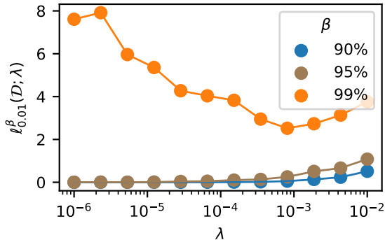
Figure 8: Relation between a regularization parameter \lambda in neural network model f^\lambda(x) , and the corresponding LAL for m \rightarrow \infty , varying \beta , and (1 - \alpha) = 99\% confidence. Appropriate regularization improves the performance in the tail of the loss distribution ( \beta = 99\% ), with an optimum around \lambda \approx 10^{-3} . The bulk of the losses ( \beta = 95\% ) are not reduced by regularization; their LAL increase with \lambda .
