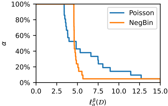
Figure 7: Comparison of models for earthquake statistics, using LAL curves and m = 1, \beta = 1 . The loss function used is the negative log-likelihood of data under the fitted model. By considering how it handles the \alpha = 20\% most difficult-to-fit data points, we see that the Negative Binomial model provides a better fit than the Poisson model.
